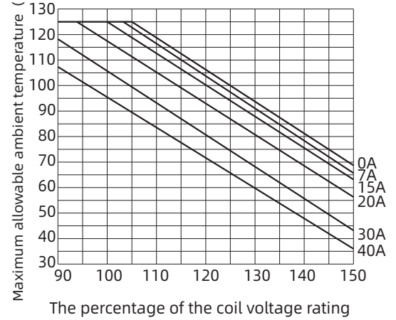
Ambient temperature vs Coil voltage
