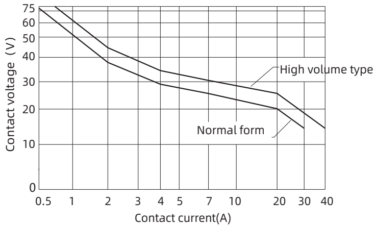
Maximum switching power
