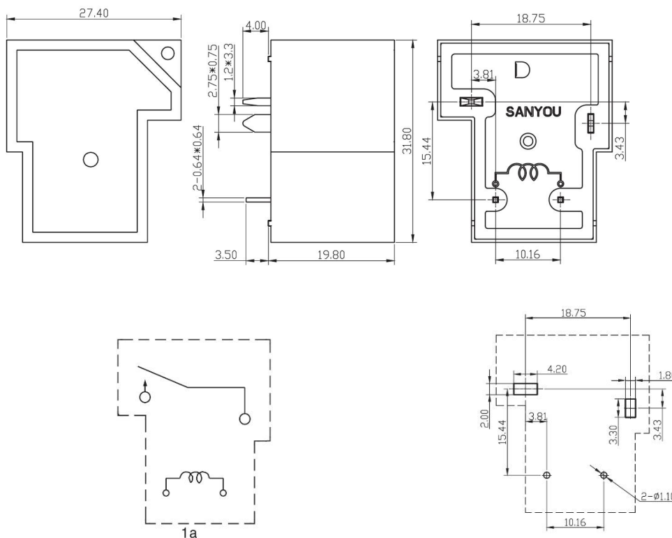
Wiring Diagram ( bottom view )
