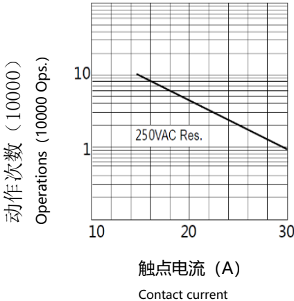
寿命曲线 Endurance Curve
