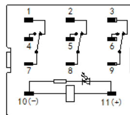
C 型带灯 C type With lamp
