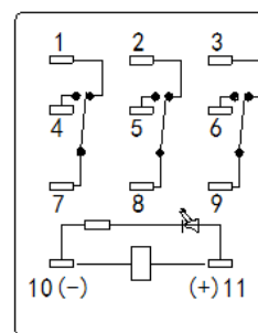
C 型带灯 C type With lamp
