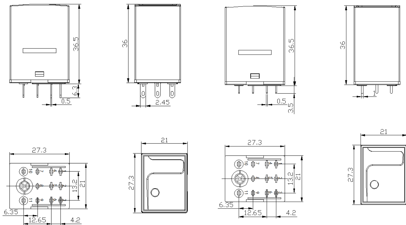
盖板型插座式 Cover plate socket type
