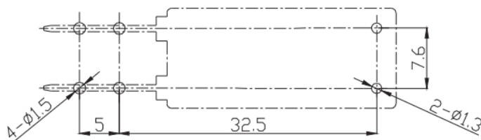
1A/1B 安装孔位图 (底视图) 1A/1B P.C.B. Layout (bottom view)
