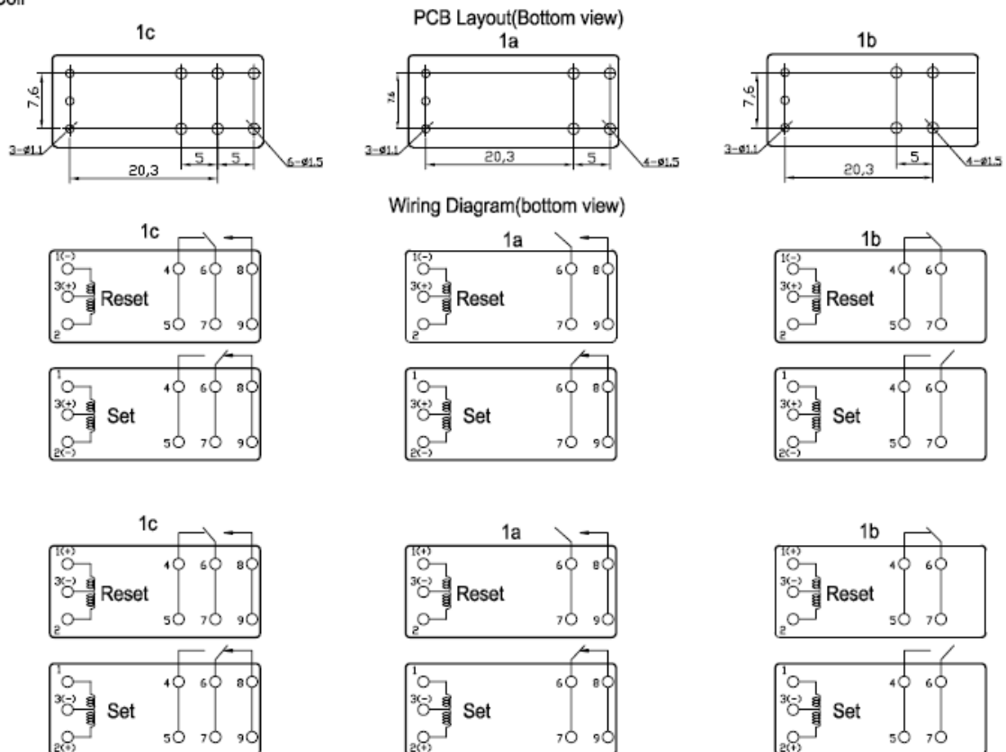
Dual Coil
