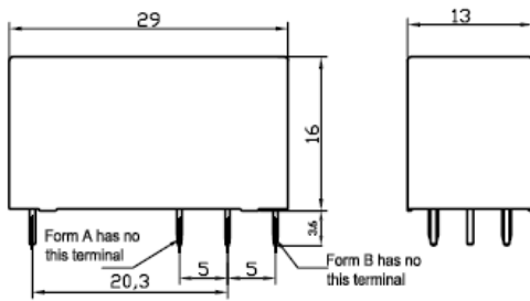
Outline Dimensions
