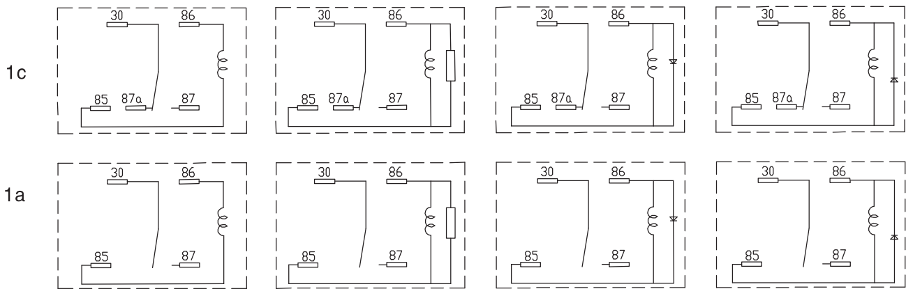
Wiring Diagram (bottom view)
